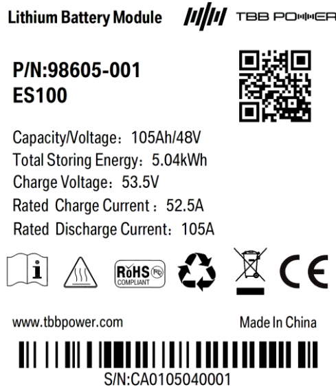
Figure 1-1 Battery Energy Storage System nameplate
