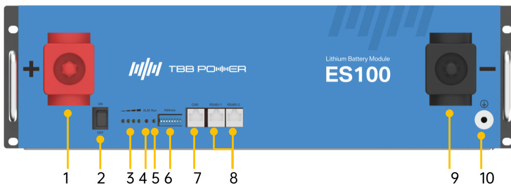
Figure 2-2 The interface of ES100
